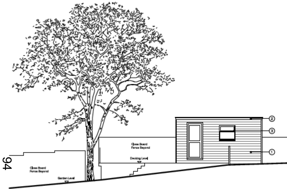
SIDE ELEVATION East
